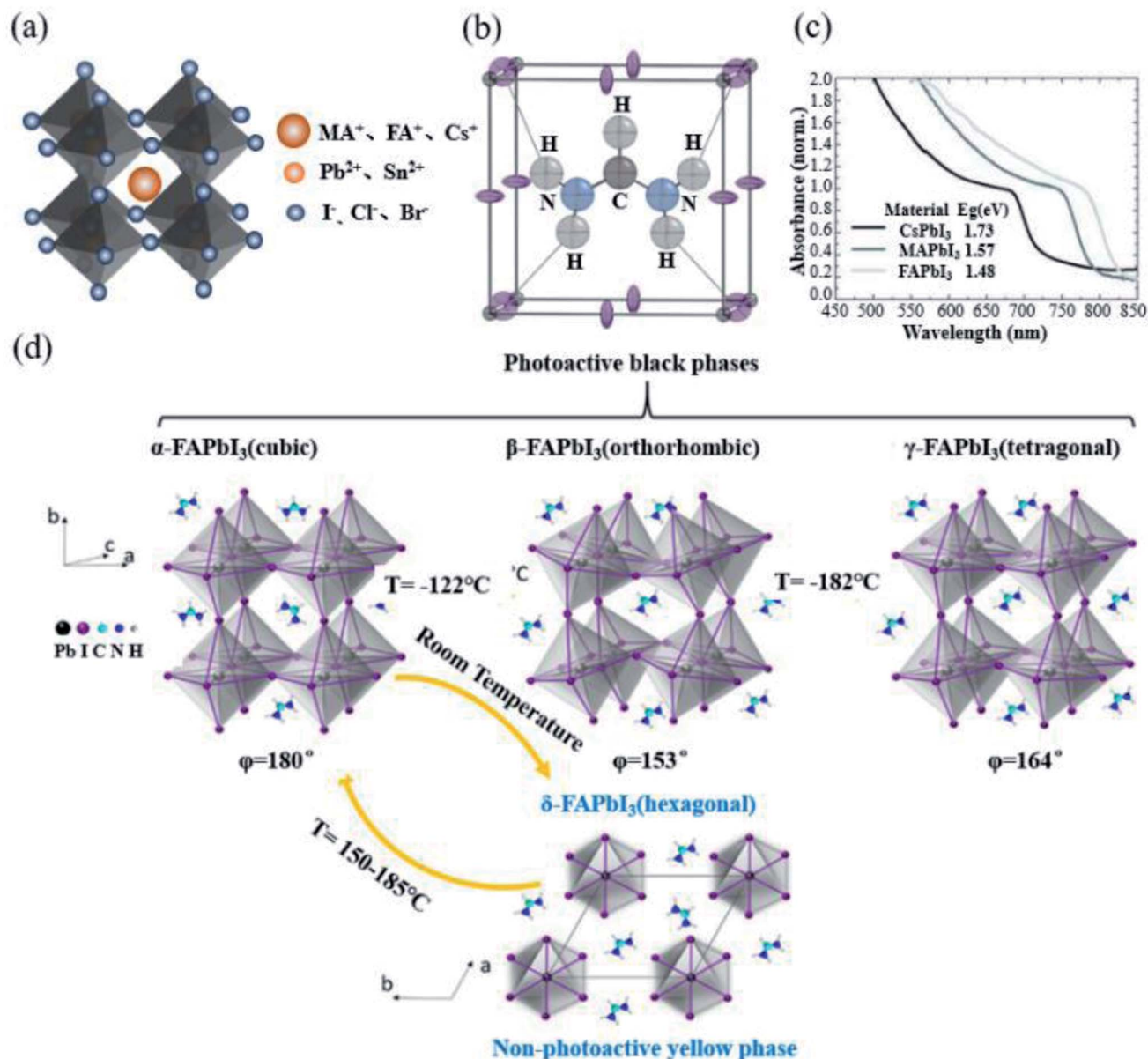
Fig. 2 (a) Schematic diagram of the crystal structure of perovskites. (b) Unit cell structure of \alpha\text{-FAPbI}_3 at 298 K. The dark gray, purple, black, blue, and pale gray spheres correspond to the Pb, I, C, N, and H atoms. NH-I hydrogen bonds are shown as dotted lines. Reprinted with permission from ref. 53, copyright 2015, American Chemical Society. (c) UV-Vis spectra for the \text{APbI}_3 perovskites formed, where A is either cesium (Cs), MA or FA. Reprinted with permission from ref. 18, copyright 2014, The Royal Society of Chemistry. (d) Crystal structure of the \text{FAPbI}_3 perovskite and phase transition between each crystal form. The common crystal structure of \text{FAPbI}_3 involves mainly \alpha and \delta phases, and \beta and \gamma phases are formed at extremely low temperatures. Reprinted with permission from ref. 54, copyright 2020, American Chemical Society.
