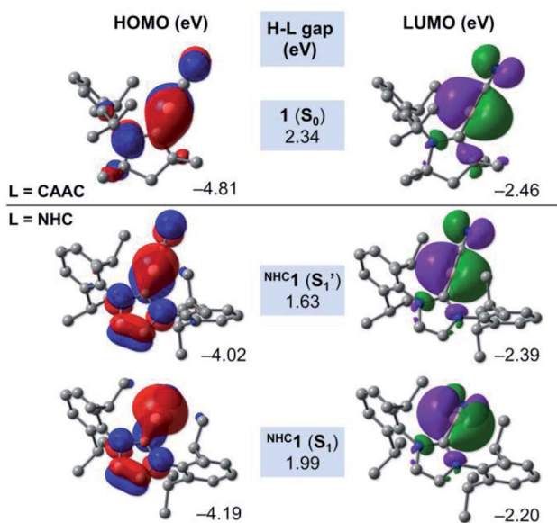
Fig. 7 Canonical Kohn–Sham frontier orbitals and H–L gaps of 1 (S_0) , NHC1 (S_1) and NHC1 (S_1') at the B3LYP–D3(BJ)/def2–SVP level of theory.
