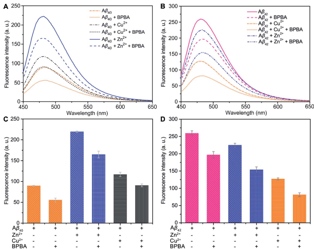
Fig. 3 ThT fluorescence intensity ( \lambda_{\text{ex}} = 415 \text{ nm} and \lambda_{\text{em}} = 485 \text{ nm} ) of \text{A}\beta_{40} (A and C) and \text{A}\beta_{42} (B and D) solutions in the absence and presence of \text{Zn}^{2+} or \text{Cu}^{2+} after incubation with or without BPBA at 37^\circ \text{C} and pH 7.4 for 24 h ( [\text{A}\beta] : [\text{metal ions}] : [\text{BPBA}] = 1 : 1 : 2 and [\text{A}\beta] = 20 \mu\text{M} ).
