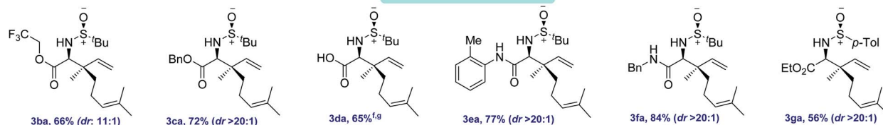
Scheme 2 Scope of allylation with \alpha -iminoesters a,b,c . a Reaction conditions: imine 1 (0.3 mmol), allylboronic acid 2 (0.39 mmol, 0.1 M in \text{CHCl}_3 ), MS 4 Å (100–150 mg) at rt under Ar. b Diastereomeric ratios (dr) were determined by ^1\text{H} NMR analysis. c Isolated yields. d Obtained as a mixture of E/Z isomers as present in commercially available farnesol. e Reactions were conducted at 60 °C. f Over two steps from glyoxalic acid. g Reaction was conducted at –30 °C.
