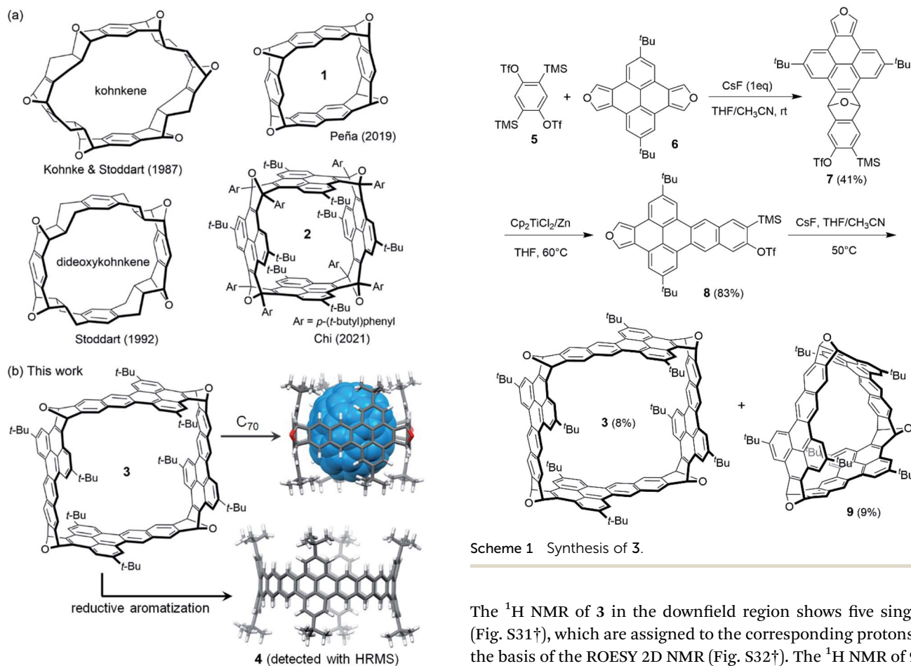
Fig. 1 (a) Structures of known oxanorbornene-fused double-stranded macrocycles; (b) structures of nanobox 3 and the energy-minimized models of carbon nanobelt 4 and C 70 C 3 as calculated at the B3LYP-D3 level of DFT with the 6-31g(d) basis set.
