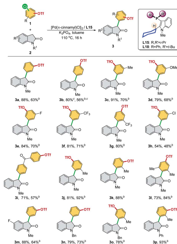
Scheme 5 Palladium-catalyzed \alpha -arylation of oxindoles through chemoselective C–Cl bond cleavage a (Reaction conditions: 1 (0.20 mmol), 2 (0.20 mmol), [Pd(\pi -cinnamyl)Cl] 2 (2 mol%), L15 (8 mol%), Pd : L = 1 : 2, K 3 PO 4 (0.40 mmol), toluene (1.0 mL), 110 °C, and 16 h. Isolated yields were reported. The chemoselectivity ratio between Ar–Cl and Ar–OTf was >99/1. b L18 was used. c Reaction conditions: 80 °C and 14 h).
