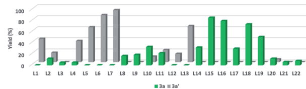
Scheme 3 Ligand screening of chemoselectivity in \alpha -arylation of N -methyl oxindole. Reaction conditions: 1a (0.20 mmol), 2a (0.20 mmol), K_3PO_4 (0.40 mmol), toluene (1.0 mL), and under N_2 . The yield was calibrated by GC-FID using dodecane as the internal standard.
