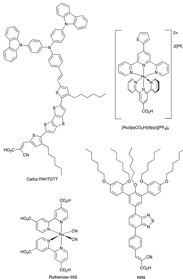
Scheme 12 Structures of the metal-free dyes Carbz-PAHTDIT and RR9, and the ruthenium(II) dyes [\text{Ru}(\text{tpyCO}_2\text{H})(\text{tppy})][\text{PF}_6]_2 ( \text{tpy} = 2,2':6',2'' -terpyridine) and the commercially available Ruthenizer-505.
