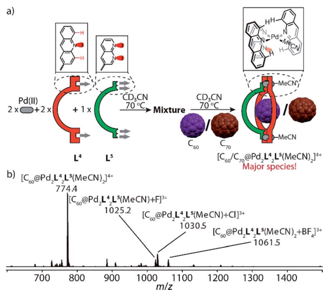
Fig. 6 Self-assembly of fullerene-containing heteroleptic bowl [\text{C}_{60}/\text{C}_{70}@\text{Pd}_2\text{L}^4_2\text{L}^5(\text{MeCN})_2] : (a) ligands L 4 and L 5 react with Pd II cations in a 2 : 1 : 2 ratio at 70 °C to give a convoluted mixture, followed by the addition of C 60 or C 70 to produce heteroleptic bowl [\text{C}_{60}/\text{C}_{70}@\text{Pd}_2\text{L}^4_2\text{L}^5(\text{MeCN})_2] as major species; (b) high-resolution ESI mass spectrum of [\text{C}_{60}@\text{Pd}_2\text{L}^4_2\text{L}^5(\text{MeCN})_2] and its anion adducts.
