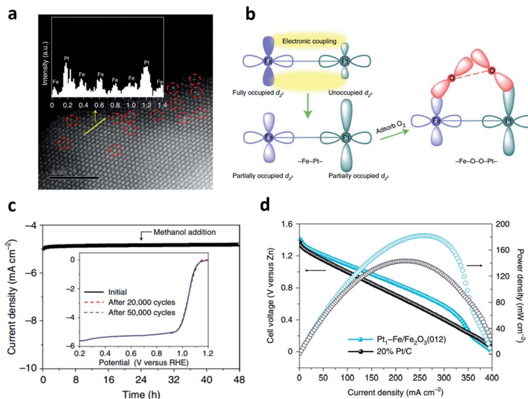
Fig. 3 (a) An aberration-corrected HAADF-STEM image ( 6 \times 6 nm 2 ) of Pt 1 -Fe/Fe 2 O 3 (012) with single-site platinum marked by red-dashed circles. (b) The schematic of the Pt–Fe electronic coupling effect for O 2 activation. (c) Chronoamperometric responses obtained at 0.90 V versus RHE at 1600 rpm. with the addition of 10 vol% methanol. The inset shows ORR polarization curves of Pt 1 -Fe/Fe 2 O 3 (012) before and after 20 000 and 50 000 voltammetry cycles. (d) Polarization and power density curves (cell voltage represents the potential versus zinc). (a–d) Reprinted with permission from ref. 45. Copyright 2021, Springer Nature.
