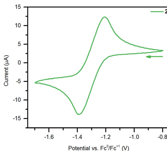
Fig. 6 Cyclic voltammogram of 2 measured in THF at 300 K (0.25 M ( n Bu 4 N)PF 6 , 1.3 mmol L -1 analyte solution, v = 50 mV s -1 ).
