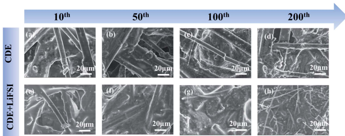
Fig. 6 SEM images of the carbon paper anode after cycling in CDE and CDE + LiFSI at the 10 th (a and e), 50 th (b and f), 100 th (c and g) and 200 th (d and h) cycles at 2C.
