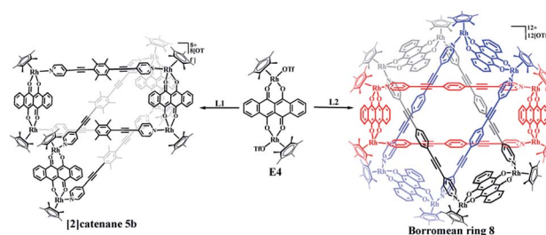
Scheme 2 Directed synthesis of [2]catenane 5b and Borromean rings 8 .
