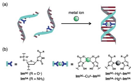
Fig. 1 (a) Schematic diagram of DNA duplexes with a metal-mediated base pair. (b) Molecular structures of novel ligand-type nucleotides bearing 2-oxo-imidazole-4-carboxylate ( Im OC ) or 2-oxo-imidazole-4-carboxamide ( Im OA ) as a nucleobase. The expected structures of metal-mediated base pairs are also shown.
