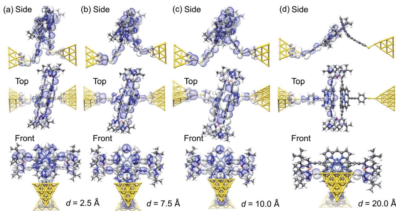
Fig. 6 (a–d), Wave function of the most transparent left-incoming transmission eigenchannel in side, top and front views for several electrode separations, d , as indicated below the panels. The transmission eigenchannels are evaluated at the Fermi energy E_F . Panel (a) belongs to a geometry in region (i), (b) to region (ii), (c) to region (iii), and (d) to region (iv), as defined in Fig. 5.
