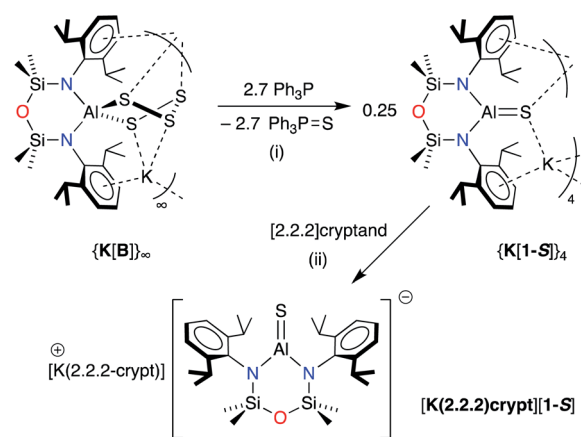
Scheme 2 Synthesis of K[Al(NON Dipp )(S)] ( K[1-S] ) and [K(2.2.2-crypt)][Al(NON Dipp )(S)] ( [K(2.2.2-crypt)][1-S] ). (i) THF solvent, crystallised from hexane; (ii) toluene solvent, crystallised from THF.
