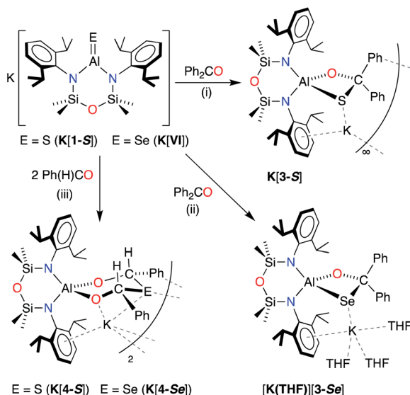
Scheme 5 Synthesis of K[Al(NON Dipp )(SC{O}Ph 2 )] ( K[3-S] ), [K(THF) 3 ][Al(NON Dipp )(SeC{O}Ph 2 )] ( [K(THF) 3 ][3-Se] ) and K[Al(NON Dipp )((OCHPh) 2 E)] (E = S, K[4-S] ; E = Se, K[4-Se] ). (i) Et 2 O solvent, crystallised from Et 2 O. (ii) THF solvent, crystallised from THF. (iii) Benzene solvent, crystallised from toluene.
