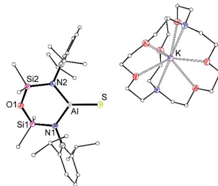
Fig. 3 Displacement ellipsoid plot (30%) of [K(2.2.2\text{-crypt})][Al(NON^{Dipp})(S)] , [K(2.2.2\text{-crypt})][1-S] . H-atoms and THF solvate omitted; C-atoms reduced for clarity. Selected bond lengths (Å) and angles ( ^\circ ): Al–S 2.0760(11), Al–N1 1.827(3), Al–N2 1.838(2). N1–Al–N2 106.22(12), N1–Al–S 126.44(9), N2–Al–S 127.34(9).
