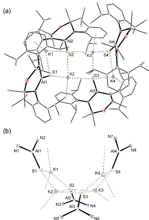
Fig. 2 (a) Displacement ellipsoid plot (30%) of [\text{K}\{\text{Al}(\text{NON}^{\text{Dipp}})(\text{S})\}]_4 , [K[1-S]] 4 . H-atoms omitted; C-atoms reduced for clarity; (b) view illustrating the ' \text{S}_4\text{K}_4 ' core.
