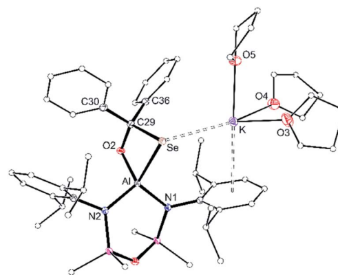
Fig. 7 Displacement ellipsoid plot (30%) of [K(THF)_3][Al(NON^{Dipp})(SeC(O)Ph_2)] ( [K(THF)][3-Se] ). H-atoms omitted; C-atoms reduced for clarity. Selected bond lengths (Å) and angles (°): Al–Se 2.4255(5), Al–O2 1.7687(12), C29–O2 1.3983(19), C29–Se 2.0484(16), Al–N1 1.8526(13), Al–N2 1.8477(14), K⋯Se 3.3501(4), Se–Al–O2 79.79(4), Al–Se–C29 69.19(5), Al–O2–C29 107.24(10), Se–C29–O2 103.52(10), N1–Al–N2 106.20(6).
