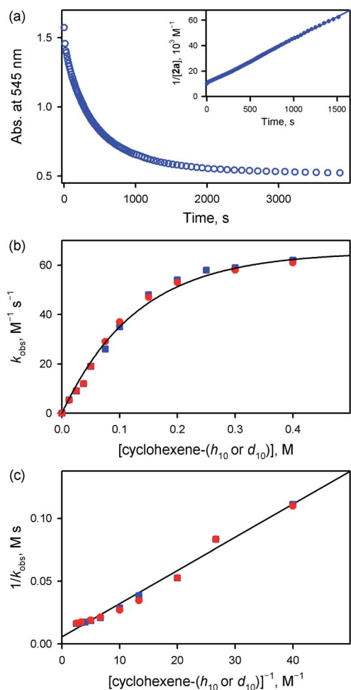
Fig. 4 (a) Time profile of the absorbance change at 545 nm due to the decay of 2a (0.10 mM) in the reaction of 2a with cyclohexene (100 mM) in butyronitrile at 253 K. Inset shows the second-order plot of 1/[2a] vs. time. (b) Plots of the observed second-order rate constants ( k_{\text{obs}} ) against concentrations of cyclohexene- h_{10} (blue squares) and cyclohexene- d_{10} (red circles) obtained in the reactions of 2a (0.10 mM) with cyclohexene- h_{10} and cyclohexene- d_{10} in butyronitrile at 253 K, respectively. (c) Plots of k_{\text{obs}}^{-1} vs. [\text{cyclohexene-}h_{10}]^{-1} (blue squares) and [\text{cyclohexene-}d_{10}]^{-1} (red circles) obtained in the reactions of 2a (0.10 mM) with cyclohexene- h_{10} and cyclohexene- d_{10} in butyronitrile at 253 K, respectively.
