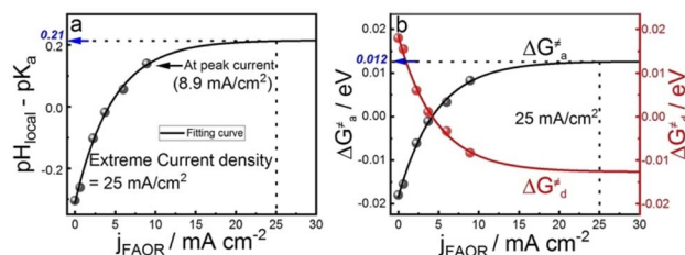
Fig. 5 The dependence of the (a) pH local - pK a of 4MPy and (b) ΔG a ‡ , ΔG d ‡ of proton transfer on the current densities.
