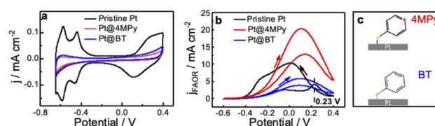
Fig. 1 Cyclic voltammograms at 0.1 V s −1 on pristine Pt (black curve), Pt@4MPy (red curve) and Pt@BT (blue curve) in 0.5 M H 2 SO 4 and (b) in 0.5 M H 2 SO 4 + 0.5 M HCOOH. The scheme of 4MPy and BT on Pt is described in (c). The current density was calculated using the geometric area of the Pt electrode to reflect the effect of 4MPy.
