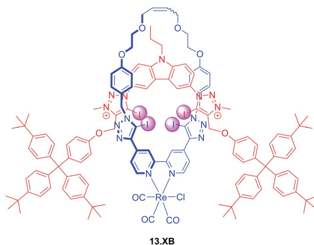
Fig. 16 All XB Re(i)(CO) 2 Cl-containing [2]rotaxane 13.XB for selective fluorescent halide sensing in ACN/ \text{H}_2\text{O} mixtures.
