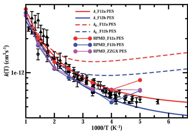
Fig. 4 Thermal rate constants of the HCl + OH \rightarrow H 2 O + Cl reaction calculated on both the F12a and F12b PES, compared with rate constants for the ground rovibrational state, the RPMD rates on ZZGX PES and the previous experimental measurements. 21,22,24–29 Experimental data are taken from Husain et al. (in circles), 21,22 Molina et al. (in diamonds), 24 Ravishankara et al. (in upward-pointing triangles), 25 Smith et al. (in squares), 26 Sharkey et al. (in triangle left), 27 Battin-Leclerc et al. (in downward-pointing triangles), 28 and Bryukov et al. (in leftward-pointing triangles). 29
