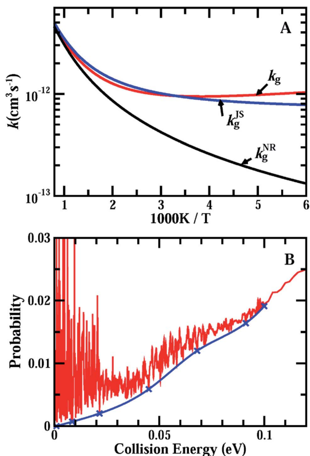
Fig. 3 (A) Accurate rate constants, k_{\text{g}} , for the initial ground rovibrational state of the \text{HCl} + \text{OH} \rightarrow \text{H}_2\text{O} + \text{Cl} reaction calculated on the F12b PES, in comparison with k_{\text{g}}^{\text{JS}} (obtained using the J -shifting approximation) and k_{\text{g}}^{\text{NR}} (based on the background reaction probabilities for J = 0 with the resonance contribution removed shown below); (B) the background reaction probabilities up to E = 0.1 eV by connecting some valleys of the reaction probabilities marked by x .
