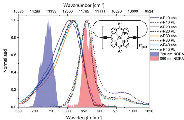
Fig. 1 Normalised steady-state absorption (solid lines) and photoluminescence (dashed lines, excitation at 750 nm) of c -P10 (violet) c -P20 (navy), c -P30 (orange) and c -P40 (teal). The normalised pump pulse spectra are shown as blue (720 nm) and red (860 nm) shaded areas. A sketch of the molecular structure of the cyclic conjugated porphyrin nanorings is shown in the inset. Ar = 3,5-bis(octyloxy) phenyl.
