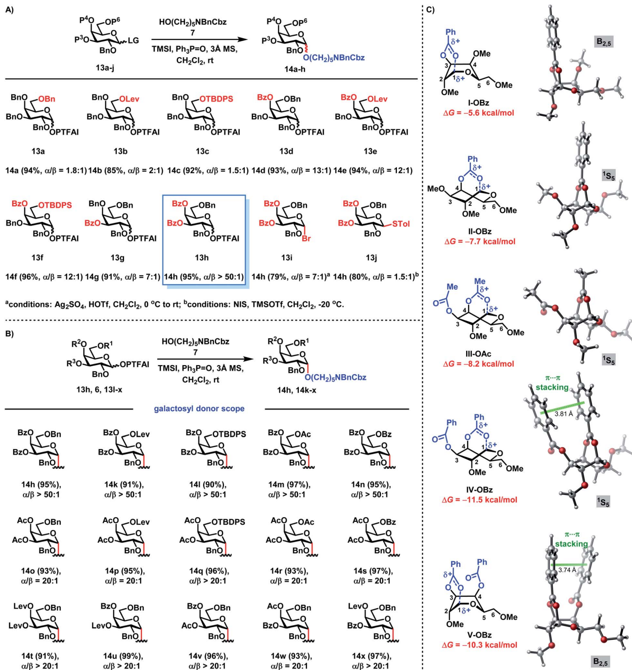
Scheme 2 (A) Reaction optimization of \alpha -galactosylation; (B) the scope of galactosyl PTFAl donors; (C) computed geometries of \beta -oxocarbenium stabilized by remote acyl groups. The relative free energies ( \Delta G ) are with respect to the oxocarbenium without the stabilization of remote acyl groups.
