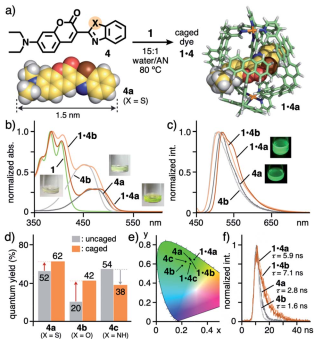
Fig. 3 (a) Formation of caged dyes 1\cdot 4 ( X = S, O, \text{ and } \text{NH} ) and the optimized structures of 4a and 1\cdot 4a ( R^1 = \text{H} for clarity). 11 (b) UV-visible spectra and photographs (r.t., 15 : 1 water/acetonitrile (AN)) of 1\cdot 4a , 1\cdot 4b , 1 , and 4a , 4b (in 2 : 1 water/AN), (c) their fluorescence spectra ( \lambda_{\text{ex}} = 450 \text{ nm} ) and (d) quantum yields, and (e) their CIE diagram (before and after binding by 1 ). (f) Fluorescence lifetimes (r.t., \lambda_{\text{ex}} = 355 \text{ nm} , 15 : 1 or 2 : 1 water/AN) of 1\cdot 4a , 1\cdot 4b , and 4a , 4b .
