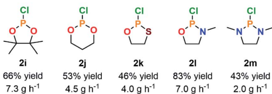
Fig. 2 Scope of cyclic adducts 2a–m obtained from the continuous flow reaction of PCl 3 with various diols and analogs through a base-free (see Table 1, entry 10) or a base-involving (see ESI, Section 2.5.2†) procedure.
