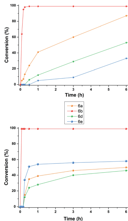
Fig. 2 Reaction progress for DA reaction between 4 and aldehydes 5a–e in the presence of: (top) 2a (26 mol%) and C 6 (26 mol%); (bottom) 26 mol% 3^+ \cdot \text{BF}_4^- .
