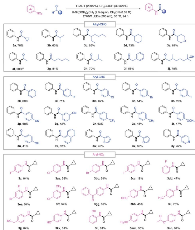
Fig. 2 Substrate scope of reductive amidation. Standard conditions: nitroarene 1 (0.1 mmol), aldehyde 2 (3 equiv.), TBADT (2 mol%), \text{CF}_3\text{COOH} (30 mol%), \text{H-Si}(\text{OCH}_2\text{CH}_3)_2\text{CH}_3 (2.5 equiv.), \text{CH}_3\text{CN} (2 mL), purple LEDs (390 nm), 30 °C, 24 h. a The amount of aldehyde was 20 equiv.
