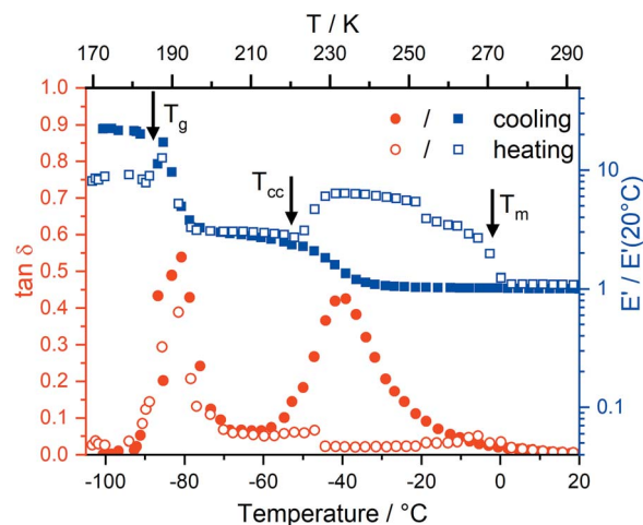
Fig. 6 Representative DMTA spectrum of [C_4C_{1im}][NTf_2] . Black arrows correspond to the thermal transitions obtained from DSC measurements. Here, f = 10 \text{ Hz} , heating (empty symbols) rate and cooling (solid symbols) rate 4 \text{ K min}^{-1} .
