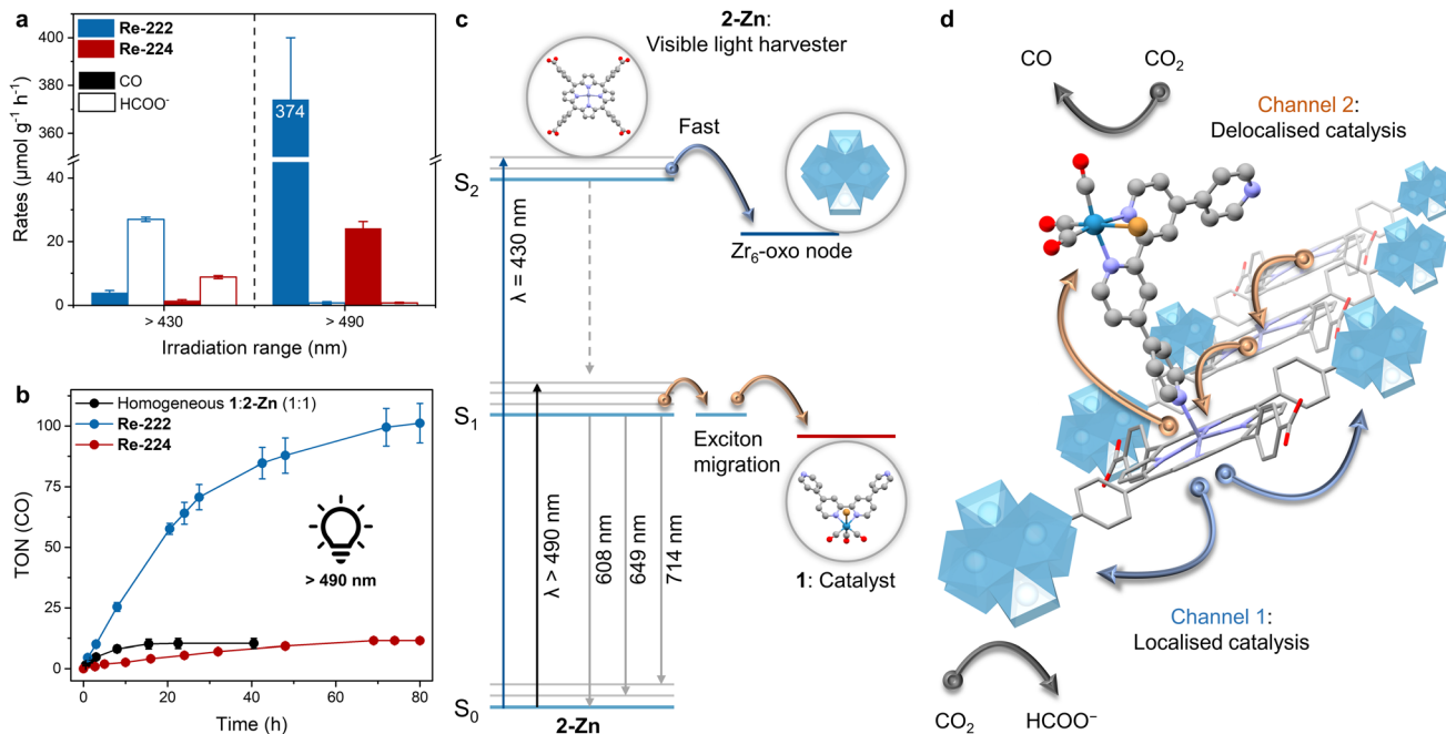
Fig. 6 Wavelength-dependent photocatalytic CO 2 reduction with Re-PCN assemblies. (a) Product evolution rates depending on irradiation wavelength averaged over the first two irradiation hours. (b) TON(CO) vs. time plot for MOF samples irradiated >490 nm. Includes the homogeneous reference (black trace). Standard conditions are MOF sample (1.5 mg) suspended in MeCN (4 mL) and deionised H 2 O (0.12 mL) with BIH (225 mg), room temperature, continuous irradiation. (c) Schematic energy level diagram illustrating the working principle upon irradiation at different wavelengths. (d) Schematic representation of the two irradiation wavelength-dependent electron channels observed in Re-PCN hybrids to either deliver localised electrons to the node for CO 2 -to-formate, or delocalised exciton migration followed by charge separation to the molecular catalyst for CO 2 -to-CO. Note that for reasons of clarity not all nodes are shown.
