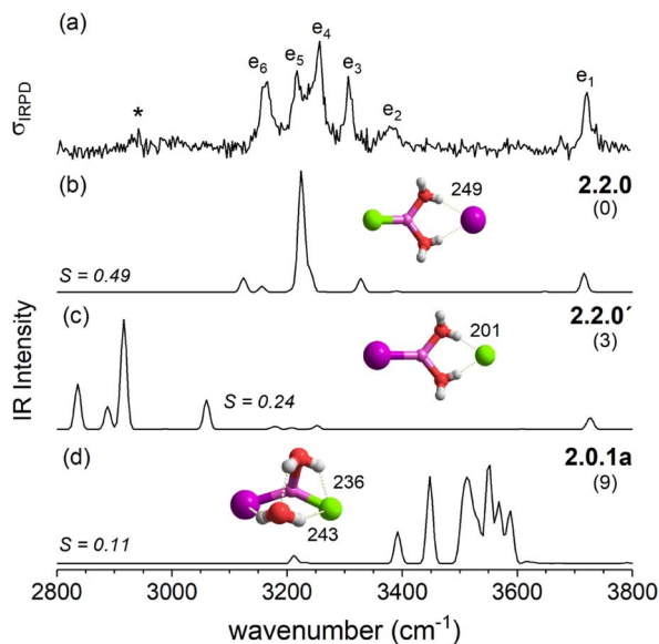
Fig. 7 Comparison of the IRPD spectrum (trace a) of D_2 -tagged [LiCl(H_2O)_2]^- to the VPT2/MP2 anharmonic spectra of the two lowest energy solvent-shared core structures 2.2.0 and 2.2.0' and intact-core structure 2.0.1a presented in traces b–d, respectively. Cosine similarity score ( S ), structures, ZPE-corrected relative energies \Delta E_0 ( \text{kJ mol}^{-1} ) and characteristic bond lengths (pm) are also shown.
