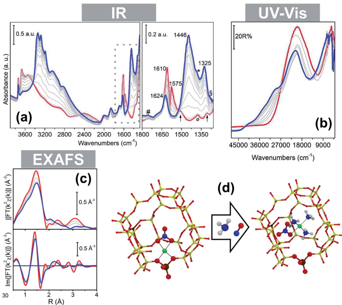
Fig. 6 In situ spectroscopy of a Cu-CHA catalyst ( \text{Si}/\text{Al} = 15 ; \text{Cu}/\text{Al} = 0.5 ) during \text{NO}/\text{NH}_3 interaction at 50 °C (grey thin and blue thick lines: intermediates and final state, respectively) after equilibration in \text{NO}/\text{O}_2 (red thick curves): (a) infrared; (b) DR UV-Vis; (c) magnitudes of FT-EXAFS spectra. (d) Structural model of a framework coordinated chelating bidentate Cu-nitrate and DFT optimized structure of the mobile mixed-ligand [\text{Cu}^{2+}(\text{NH}_3)_3(\text{NO}_3)]^+ complex in the chabazite cage. Colour code: green, Cu; yellow, Si; brown, Al; red, O; blue, N; white, H. Adapted from ref. 97 with permission from John Wiley and Sons, copyright 2019.
