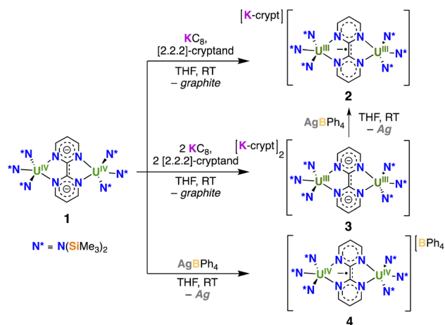
Scheme 2 Synthesis of [K(2,2,2-cryptand)][((Me_3Si)_2N)_3U]_2(\mu-bpym)] , 2 , [K(2,2,2-cryptand)]_2[(((Me_3Si)_2N)_3U)_2(\mu-bpym)] , 3 , and [BPh_4][((Me_3Si)_2N)_3U]_2(\mu-bpym)] , 4 .
