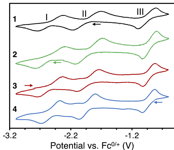
Fig. 2 Cyclic voltammograms of \{[(\text{Me}_3\text{Si})_2\text{N})_3\text{U}_2(\mu\text{-bpym})]\} , 1 (black), [\text{K}(2.2.2\text{-cryptand})]\{[(\text{Me}_3\text{Si})_2\text{N})_3\text{U}_2(\mu\text{-bpym})]\} , 2 (green), [\text{K}(2.2.2\text{-cryptand})]_2\{[(\text{Me}_3\text{Si})_2\text{N})_3\text{U}_2(\mu\text{-bpym})]\} , 3 (red), and \{[(\text{Me}_3\text{Si})_2\text{N})_3\text{U}_2(\mu\text{-bpym})][\text{BPh}_4]\} , 4 (blue), in THF/0.06 M [\text{NBu}_4][\text{BPh}_4] at a 50 \text{ mV s}^{-1} scan rate versus \text{Fc}/\text{Fc}^+ using a \text{Pt}^0 disk as a working electrode (arrows indicate scan direction).
