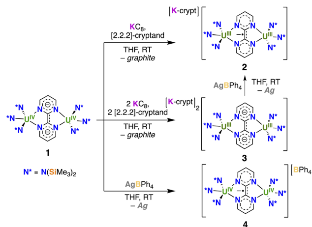
Scheme 2 Synthesis of [K(2,2,2\text{-cryptand})][((Me_3Si)_2N)_3U]_2(\mu\text{-bpym}) , 2 , [K(2,2,2\text{-cryptand})]_2[((Me_3Si)_2N)_3U]_2(\mu\text{-bpym}) , 3 , and [((Me_3Si)_2N)_3U]_2(\mu\text{-bpym})[BPh_4] , 4 .
