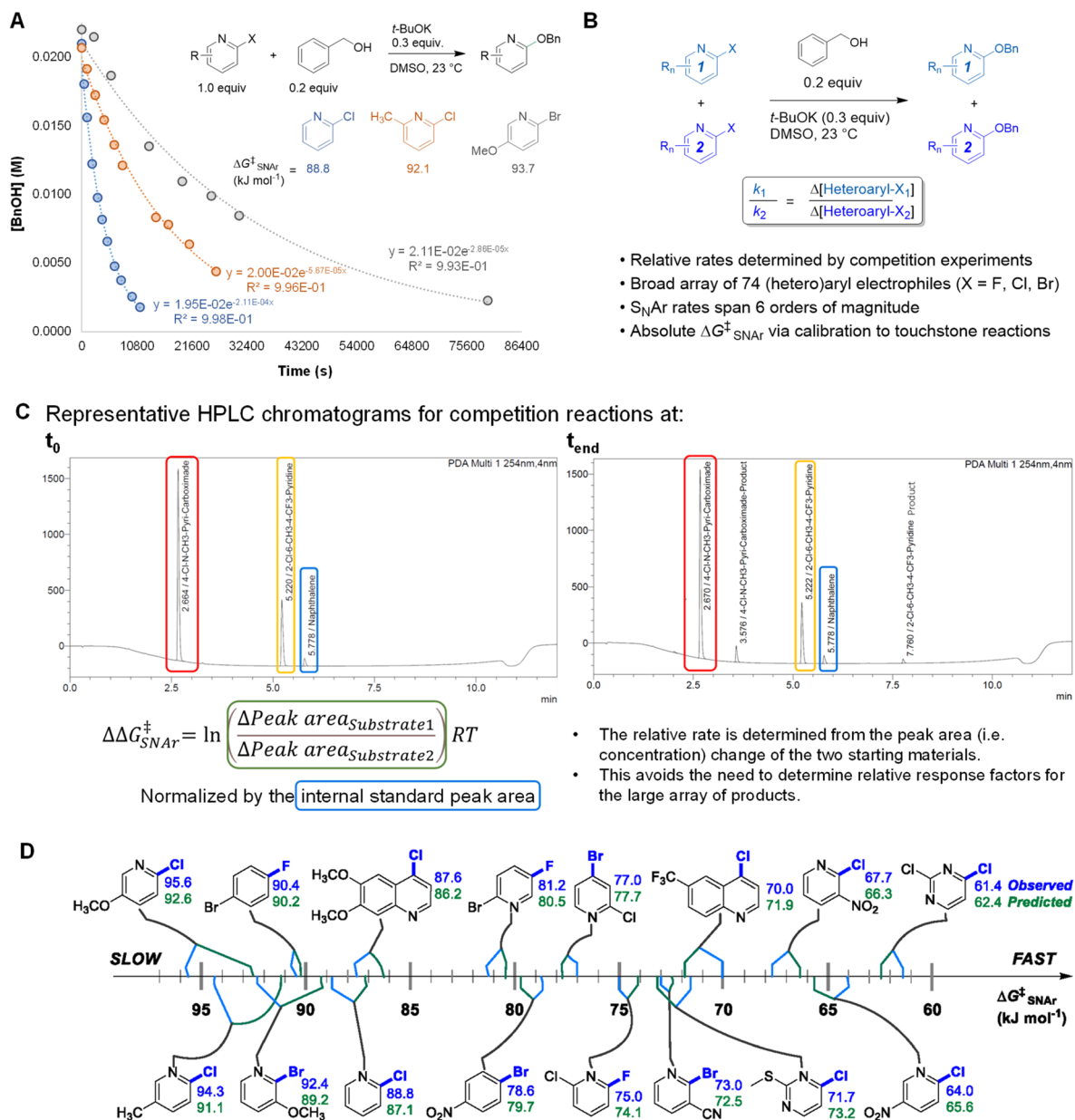
Fig. 2 Experimental approach to collecting free energies of activation for 74 \text{S}_{\text{NAr}} reactions; Bn = benzyl. (A) Touchstone reaction progress analysis under pseudo first order conditions. (B) Competition experiments to establish relative rates across electrophile library. (C) Representative primary data for determining \Delta \Delta G^\ddagger_{\text{SNAr}} from competition experiments. (D) Quantitative reactivity scale for representative electrophiles.
