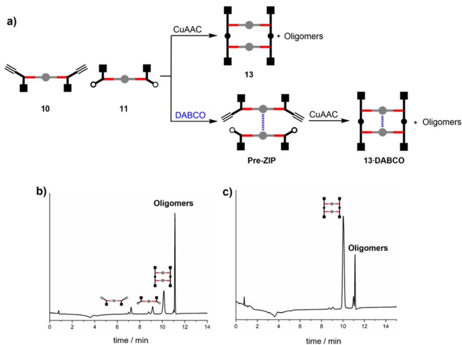
Fig. 2 (a) Reaction pathways in the CuAAC reaction between 10 and 11 in the absence or presence of DABCO. HPLC chromatograms of the product mixture obtained from reaction of 10 (15 μM), 11 (15 μM) and CuTBTA (0.02 mM) in CH 2 Cl 2 at room temperature for 16 h (b) in the absence of DABCO, and (c) in the presence of DABCO (15 μM). The sharp peak at 11 minutes corresponds to the point at which the eluant switched to 100% THF and washed all remaining species off the column.
