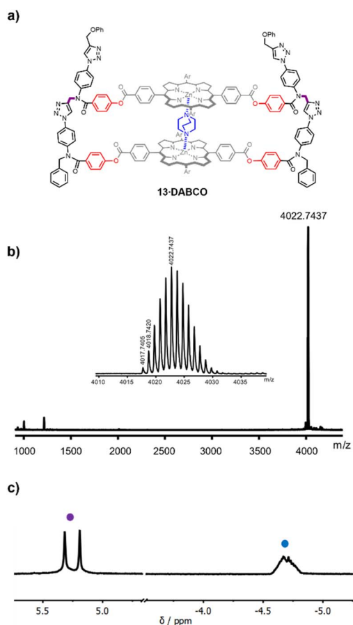
Fig. 3 (a) Chemical structure of the DABCO complex of duplex 13 . (b) MALDI-HRMS of 13 (calculated mass for [M]^+ = 4017.7608). (c) Partial 500 MHz 1 H-NMR spectrum of the DABCO complex of 13 in CDCl 3 at room temperature. The signals due to the amide NCH 2 groups (purple), and the upfield shifted signal due to bound DABCO (blue) are indicated.
