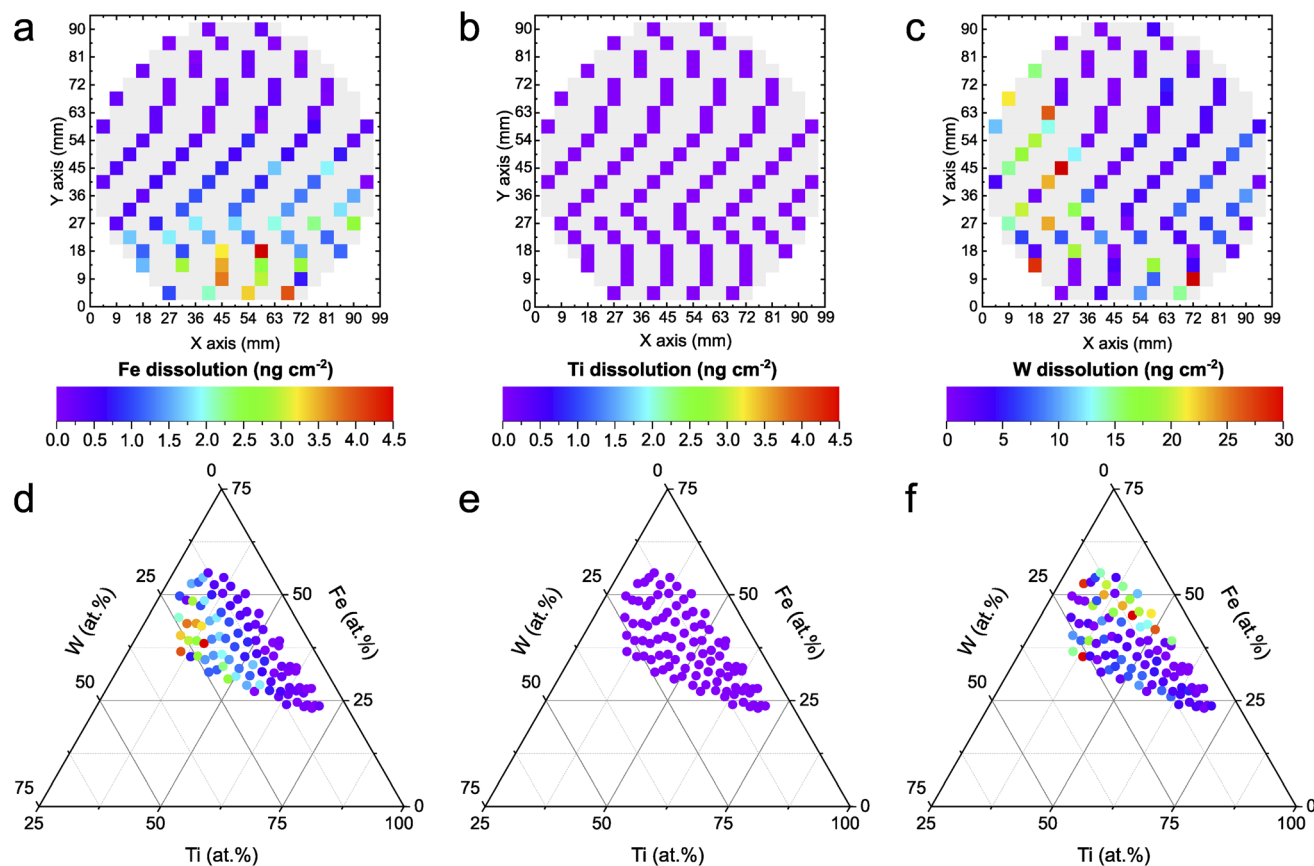
Fig. 2 Element-specific dissolution of Fe-Ti-W-O material library at 1.7 V RHE . (a-c) Dissolved amounts of Fe (a), Ti (b), and W (c) mapped onto a schematic representation of the wafer. (d-f) Dissolved amounts of Fe (d), Ti (e), and W (f) mapped onto a ternary diagram. The HT measurements were conducted in 0.05 M NaNO 3 (pH 5.7) under 1 Sun Am 1.5G illumination. Note that the color scale for W differs from Fe and Ti.
