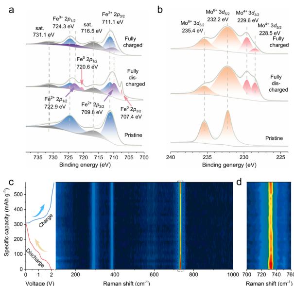
Fig. 3 (a and b) Ex situ XPS Fe 2p and Mo 3d at different discharge/charge states. (c and d) In situ Raman spectra of a P-FMO positive electrode in an AIB.
