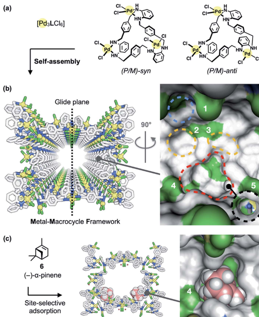
Fig. 2 Metal-macrocycle framework (MMF). (a) Self-assembly of asymmetrically twisted Pd^{II} -macrocycles into (b) a porous crystal MMF (sticks model) with five enantiomeric pairs of binding pockets (surface model). (c) Previously reported site-selective adsorption of (-)\text{-}\alpha\text{-pinene} (6) (space-filling model) on the channel surface of the MMF. 1 Blue, yellow, red, or black dashed circles indicate the ceiling-, side-, bottom-, or tubular-pockets of the MMF, respectively. MMF: Pd, yellow; Cl, green; N, blue; C, grey. 6: C, pink; H, white. Hydrogen atoms attached to the MMF were omitted for clarity. Green or blue surface represents exposed Cl or N-H groups of the MMF, respectively.
