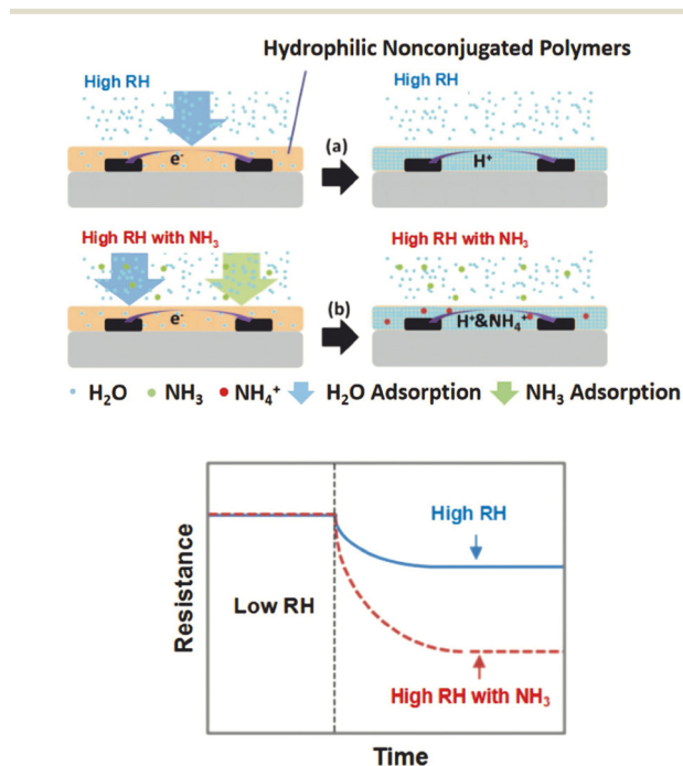
Fig. 9 Schematic showing a sensor based on hydrophilic nonconjugated polymers responding to a) a high RH and b) a high RH and ammonia. These sensors make use of high levels of humidity to increase the sensor response by using the water to absorb and ionise the ammonia, rather than viewing high levels of humidity as a disadvantage. Reproduced with permission from Zhao 2020. 57
