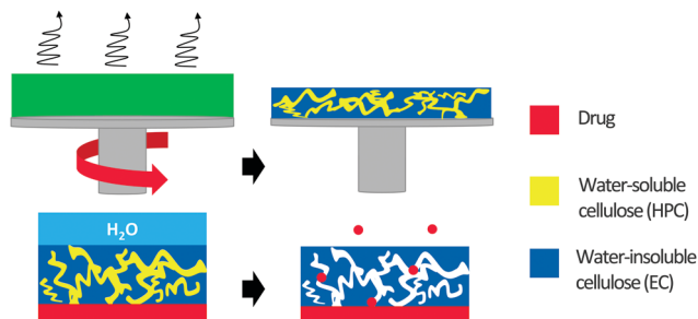
Fig. 1 Illustration of the formation of a porous phase-separated film made of EC and HPC using spin coating with evaporation of ethanol and kinetic trapping (top). With subsequent leaching of the water-soluble HPC phase (bottom left), such a coating around a drug pellet facilitates controlled release of the drug (bottom right).
