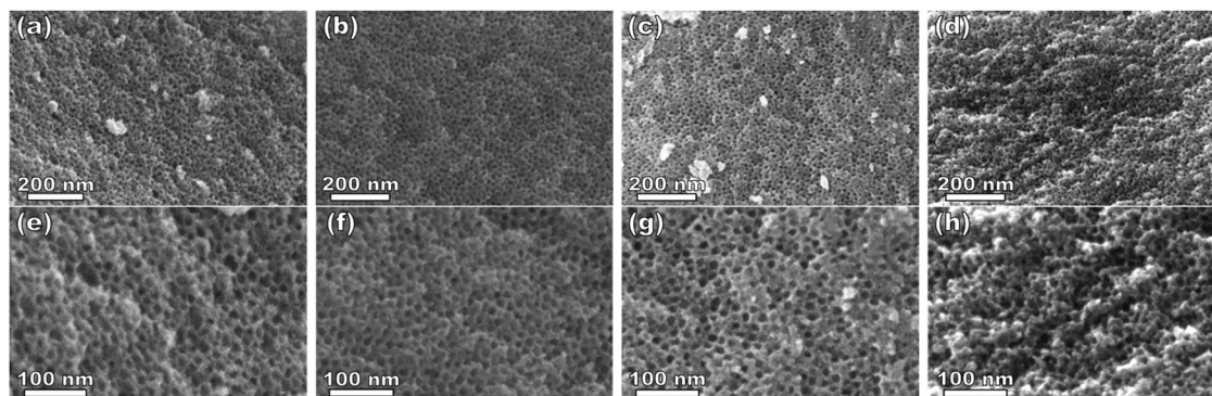
Fig. 9 SEM images of bulk titania samples prepared by casting \text{O}_{45}\text{F}_{11} micelle templates with material precursors. The images are arranged in order of increasing material-to-template ratios: 1.50 (a and e), 3.00 (b and f), 3.50 (c and g), 4.00 (d and h).
