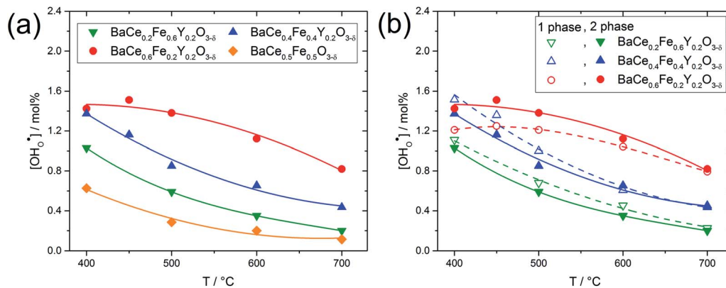
Fig. 5 (a) Proton concentrations of two-phase composites with frozen-in oxygen stoichiometry in 17 mbar p_{\text{H}_2\text{O}} (samples were quenched from 700 ^{\circ}\text{C} in \text{N}_2 ) as a function of temperature. (b) Comparison of the proton concentration of two-phase composites (samples sintered at temperatures below the upper critical mixing temperature; closed symbols and full lines) and the corresponding single phases (samples sintered at temperatures above the upper critical mixing temperature; open symbols and dashed line). The lines are guidelines to the eye.
