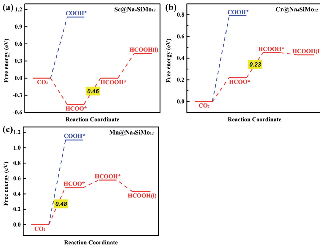
Fig. 6 Calculated free energy diagrams for the electrochemical \text{CO}_2\text{RR} on (a) \text{Sc}@Na_4SiMo_{12} , (b) \text{Cr}@Na_4SiMo_{12} and (c) \text{Mn}@Na_4SiMo_{12} .
