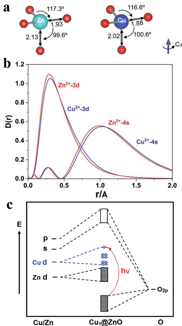
Fig. 6 (a) The local C_{3v} ligand field of ZnO and doped Cu_1@ZnO surface in crystal (color code: Cu-blue, O-red, Zn-green). (b) The radial distribution probability density ( D(r) = r^2R(r)^2 ) of atomic orbitals (AOs) of Zn(II) and Cu(II); (c) schematic energy levels of the Cu_1@ZnO single-atom catalyst.
