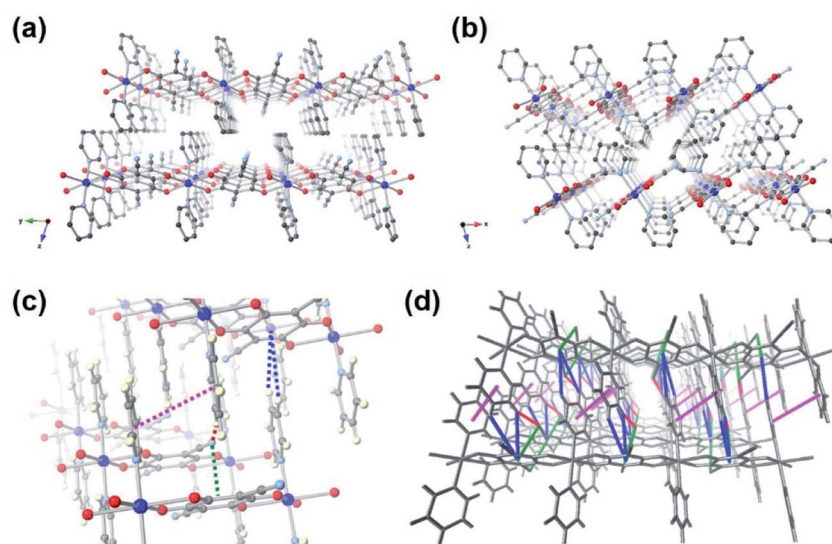
Fig. 1 (a) and (b) The single crystal structure of [\text{CuL}(\text{Py})_2]_n viewed along the x -axis and y -axis, respectively. The hydrogen atoms are omitted for clarity. (c) Packing of [\text{CuL}(\text{Py})_2]_n by supramolecular \text{C}\equiv\text{N}\cdots\pi (green dotted line), \text{C}\equiv\text{N}\cdots\text{H} (red dotted lines), \text{C}-\text{H}\cdots\pi (blue dotted lines) and \pi\cdots\pi (magenta dotted line) interactions. Colours of atoms: blue: \text{Cu}(\text{II}) ; grey: C; red: O; cyan: N; white: H. (d) The perspective view of supramolecular network in [\text{CuL}(\text{Py})_2]_n . The structure of [\text{CuL}(\text{Py})_2]_n is grayed for clarity.
