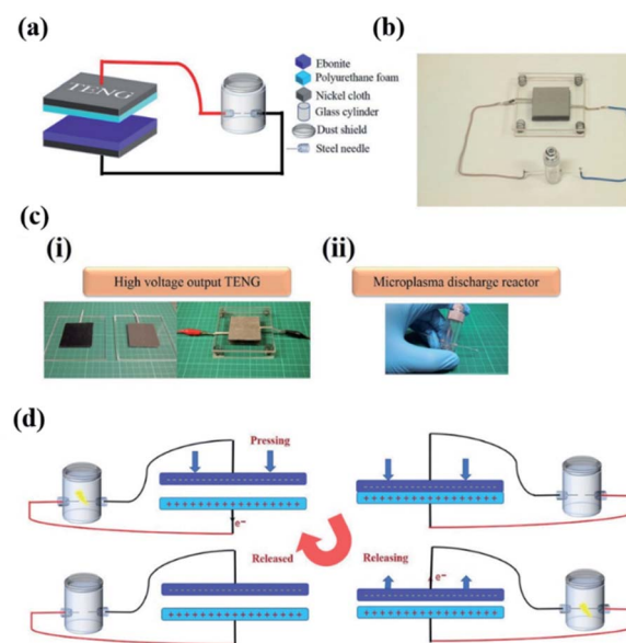
Fig. 1 Illustration of the hybridized TENG and the micro-plasma discharge system. (a) Schematic and (b) real pictures of the integrated nitrogen fixation system. (c) Real pictures of the (i) TENG and (ii) micro-plasma discharge reactor. (d) Schematic diagram of the working mechanism of the TENG and the energy supply to the micro-plasma nitrogen fixation system. Reproduced with permission. 33 Copyright 2019, Wiley VCH.
