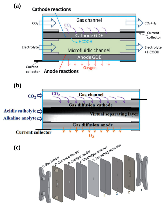
Fig. 10 (a) Schematic diagram of a microfluidic flow cell. Adapted with permission. 183 Copyright 2012, Elsevier. (b) Schematic diagram of a dual electrolyte microfluidic flow cell. Adapted with permission. 180 Copyright 2016, Elsevier.
