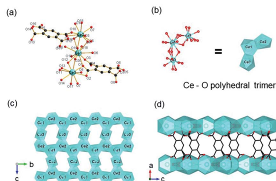
Fig. 13 (a) The coordination environment of Ce(III) ions among CTH-15; (b) the structure of Ce–O polyhedral trimer via face-sharing; (c) the 2D structure of CTH-15 growing within the b – c plane; (d) the channel distribution of CTH-15 projected along the b -axis. Reproduced with permission from ref. 21. Copyright 2021, Elsevier Inc.
