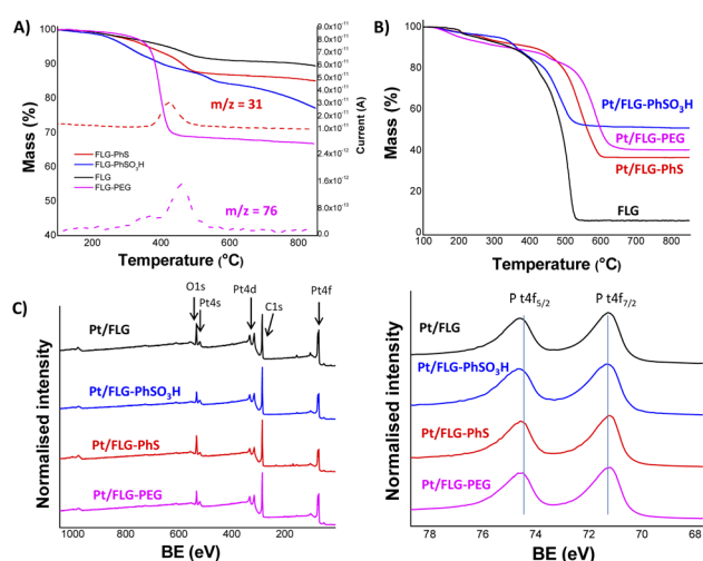
Fig. 1 Characterisation of functionalised graphene samples. (A) TGA-MS under N 2 of functionalised graphene samples. Phenyl and PEG fragments m/z = 76 (C 6 H 4 + ) and m/z = 31 (CH 3 O + ), respectively. (B) TGA under air of platinum supported graphene samples. (C) XPS spectra of platinum supported graphene samples (left panel) and platinum Pt 4f component (right panel).
