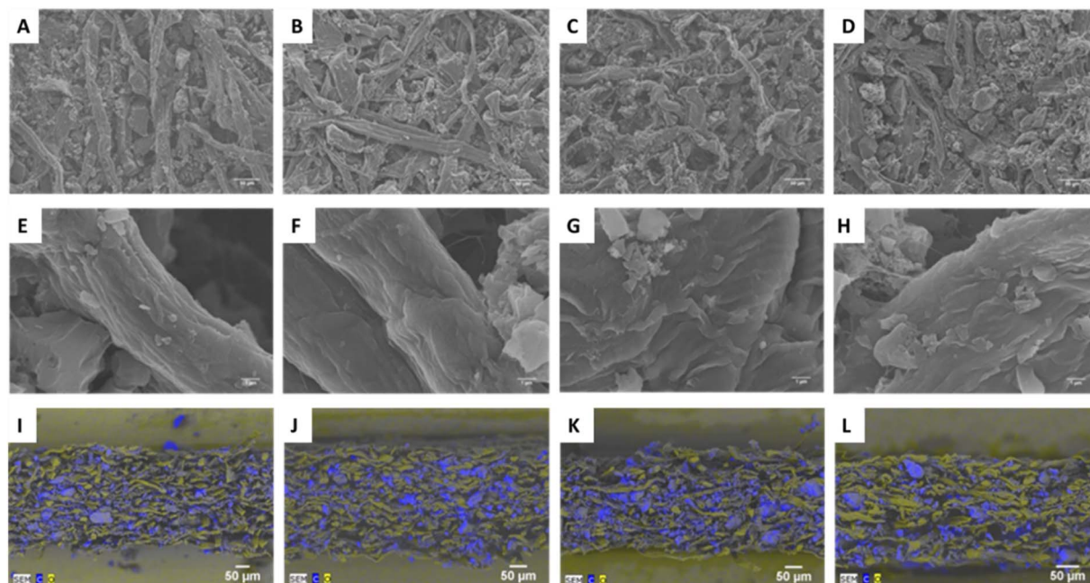
Fig. 2 Scanning electron microscopy images of the paper electrodes. SEM images of papers (top), zoom-in images of fiber surface (middle) and cross-section SEM/EDX images (bottom) of the papers made from formulations (i) (A, E and I), (ii) (B, F and J), (iii) (C, G and K) and (iv) (D, H and L). On the EDX maps, the oxygen-rich cellulose fibers appear yellow while the carbon-rich AC and CB filler particles appear blue. More aggregated structures can be observed for formulations (ii) and (iv), and a skewed filler distribution profile can be observed for formulation (ii) in the cross-section (J).
