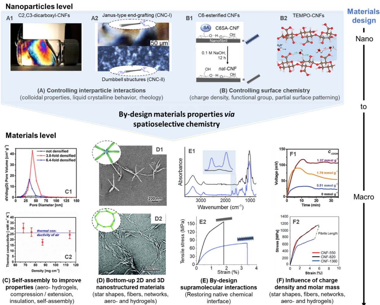
Fig. 9 Influence of spatioselective modification of nanocelluloses on nanoparticle and materials properties. C 2 , C 3 -dicarboxyl-CNFs (produced by sequential periodate and Pinnick oxidation) forms highly ordered CNF dispersions (A 1 ), which can be processed into aerogels with controlled porosity and alignment (C 1 ) to enable optimal thermal insulation behavior (C 2 ). Anisotropic and isotropic end-group grafting of CNCs can be used to influence their order in liquid crystalline films (A 2 ), and enable self-assembly into star-shaped (D 1 ) or network-like superstructures (D 2 ). Reversible succinylation at the C 6 -OH enables individualization into CNFs and is reversible to restore the native chemical interface of cellulose (B 1 ). This can be used to produce highly stiff nanopapers of assembled native CNFs (E 1 and E 2 ). TEMPO-CNFs and their regularly patterned carboxyl moieties enable, e.g., high ion conductivity (B 2 ), and allow straight-forward tuning of their degree of oxidation for optimal electricity generation (F 1 ), as well as to limit polymer degradation for the production of ultra-strong fibers (F 2 ). (A 1 ), (C 1 ), and (C 2 ) were adapted with permission from Plappert et al. 104 Copyright 2017 American Chemical Society. (A 2 ) was adapted with permission from Delépierre et al. 182 Copyright 2021 American Chemical Society. (D 1 ) was adapted with permission from Lin et al. 200 Copyright 2019 American Chemical Society. (D 2 ) was reproduced from Lin et al. 167 with permission from Royal Society of Chemistry. (B 1 ), (E 1 ), and (E 2 ) were adapted with permission from Beaumont et al. 90 under CC BY 4.0. Copyright 2021 American Chemical Society. (B 2 ) was adapted with permission from Bayer et al. 215 Copyright 2017 American Chemical Society. (F 1 ) was reprinted with permission from Li et al. 216 Copyright 2019 Wiley. (F 2 ) was reprinted with permission from Mittal et al. 217 Copyright 2018 American Chemical Society. †
