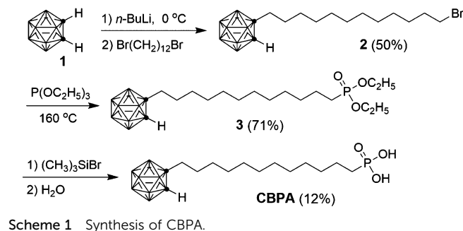
Scheme 1 Synthesis of CBPA.
