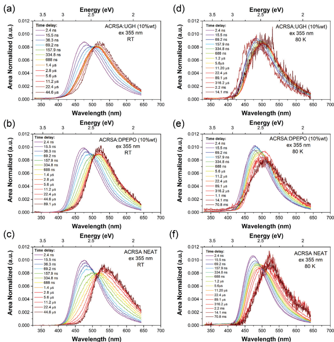
Fig. 4 Time evolution of the emission spectra (area normalised). Laser excitation at 355 nm excitation wavelength, for ACRSA in UGH, DPEO (10% loading) and neat film measured at; (a–c) 300 K, (d–f) at 80 K. Normalised data shown in Fig. S25 (ESI†).
